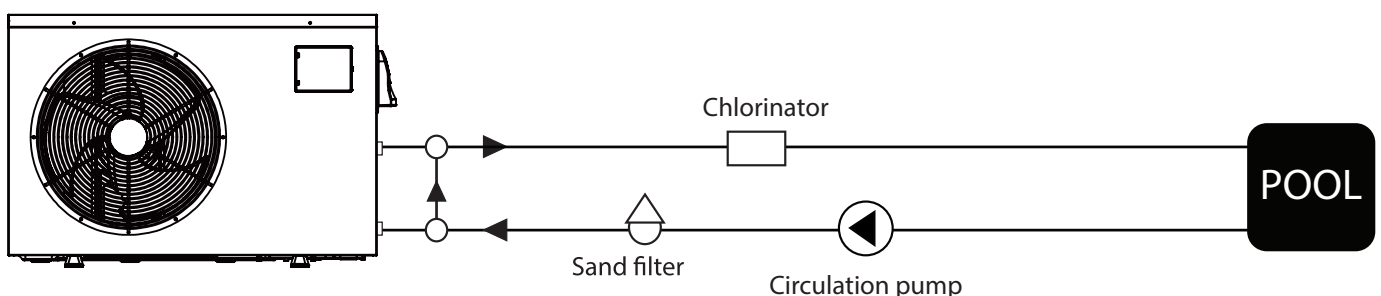
Outline diagram for installation of BONUM-series
